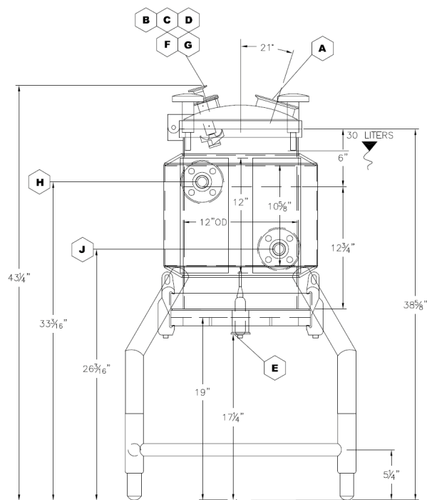
ELEVATION VIEW
