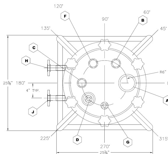
PLAN VIEW (SHOWS TRUE ORIENTATION)
