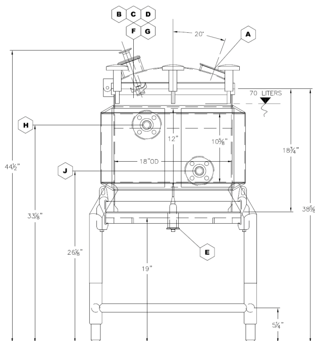
ELEVATION VIEW
