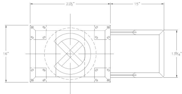
CART PLAN VIEW (SHOWS TRUE ORIENTATION)
